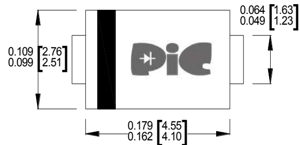
SMA/ DO-214AC
